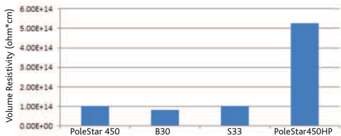
Volume Resistivity At room temperature
