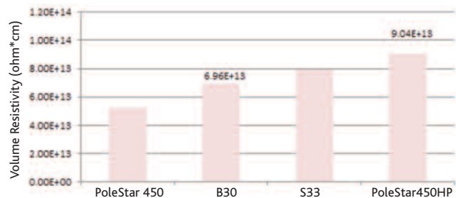
Volume Resistivity Water aged at 90 deg C for 7 days
